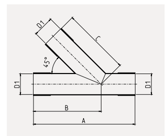
Branch pipe K45
