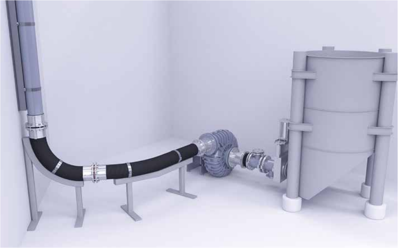
Principle figure showing Metso slurry hose system with support beam.
